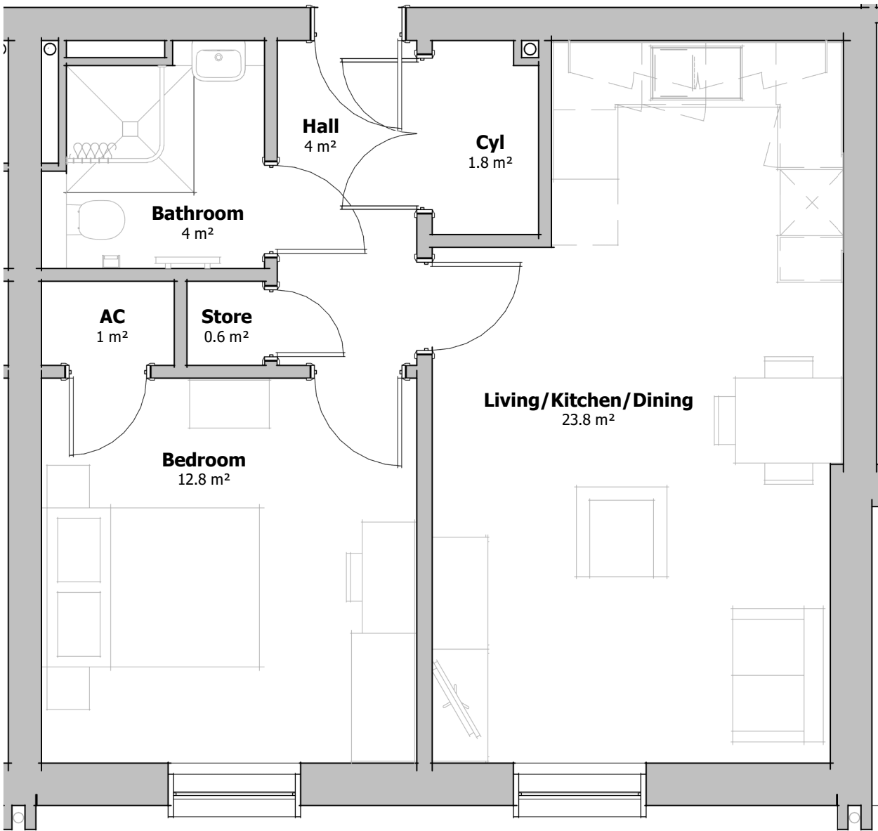
PROPOSED - TYPICAL APARTMENT PLAN 1 : 50
