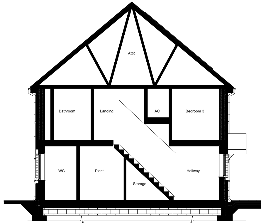
Building Section
