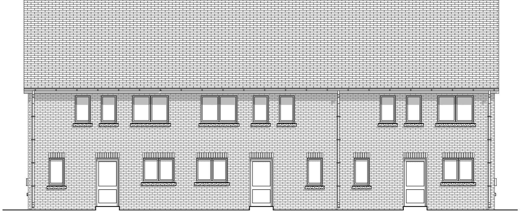
Rear Elevation
