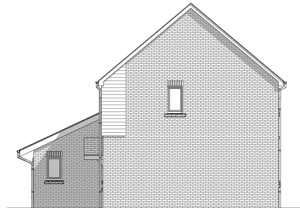
Right-Side Elevation
