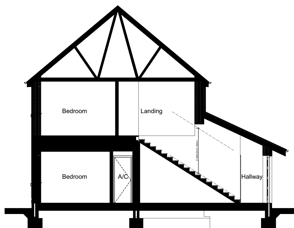
Building Section
