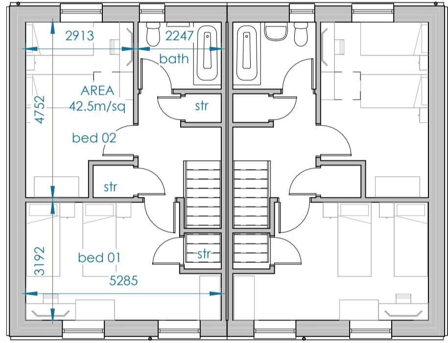
2 SEMI B FIRST 1 : 100
