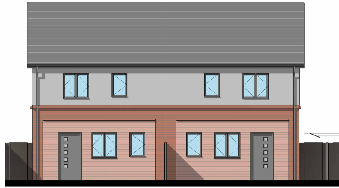
4 SEMI B ELEVATION REAR 1 : 100
