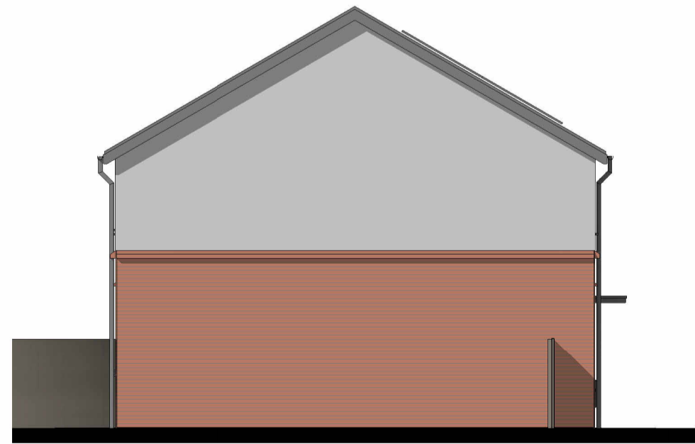
6 SEMI B ELEVATION SIDE B 1 : 100
