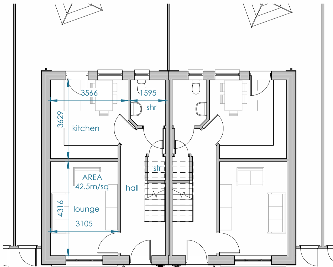
1 SEMI B GROUND 1 : 100
