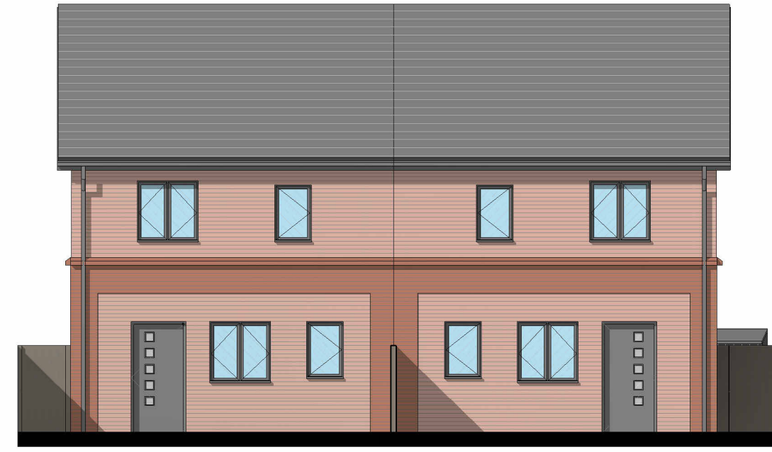
4 SEMI A ELEVATION REAR 1 : 100
