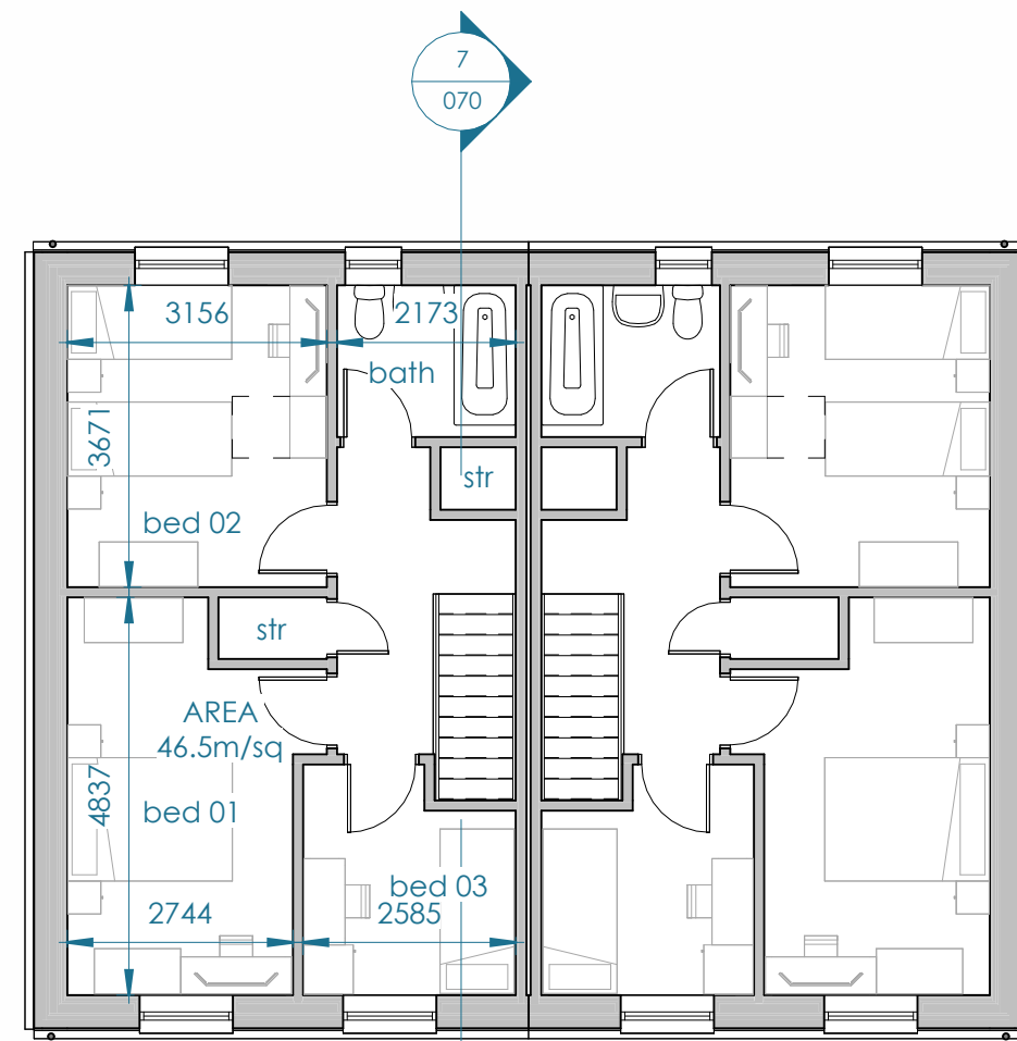
2 SEMI A FIRST 1 : 100
